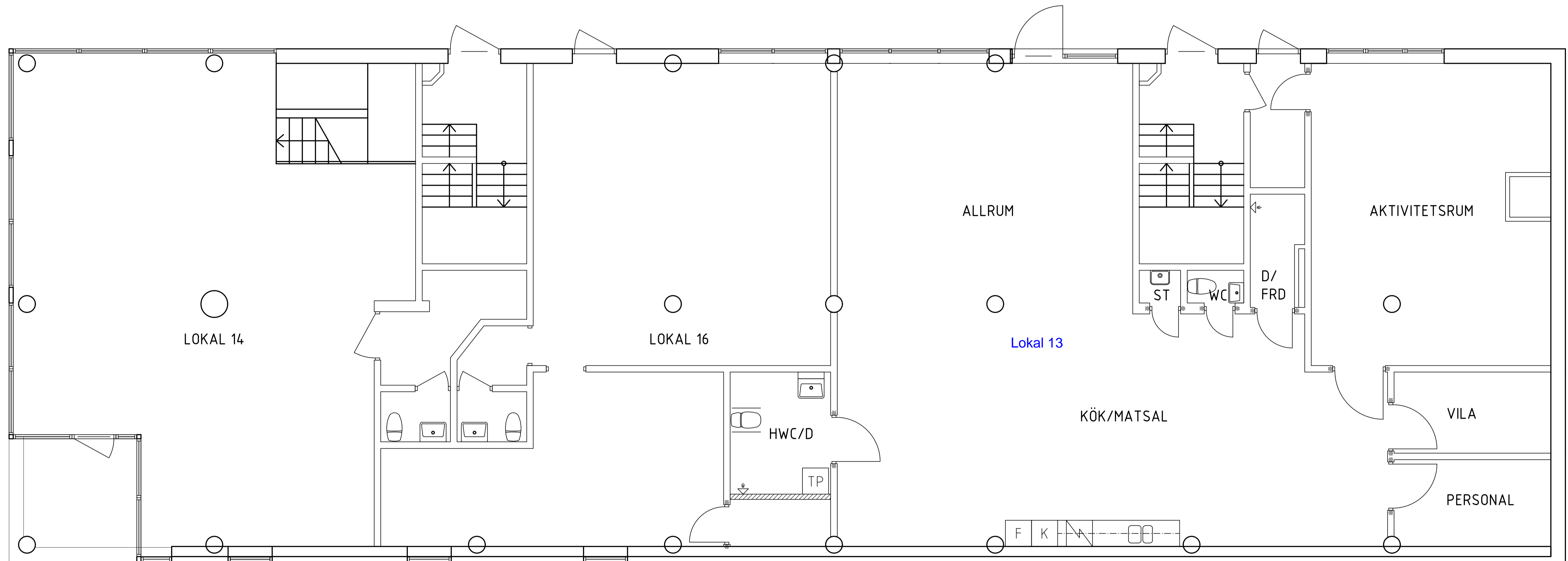
BOTTENPLAN
